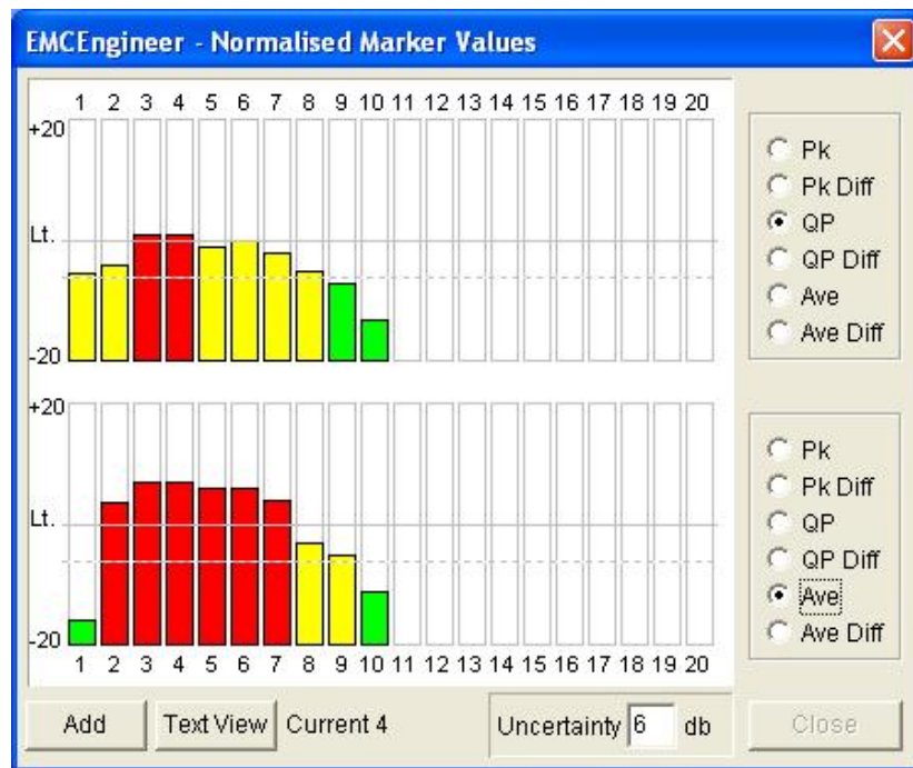
Fig 7. bargraph presentation
