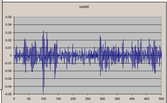
Plot sc1004 shows the ambient as output from the log periodic antenna
