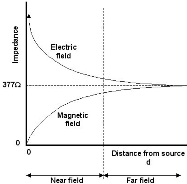
Fig 2. Field Impedance
